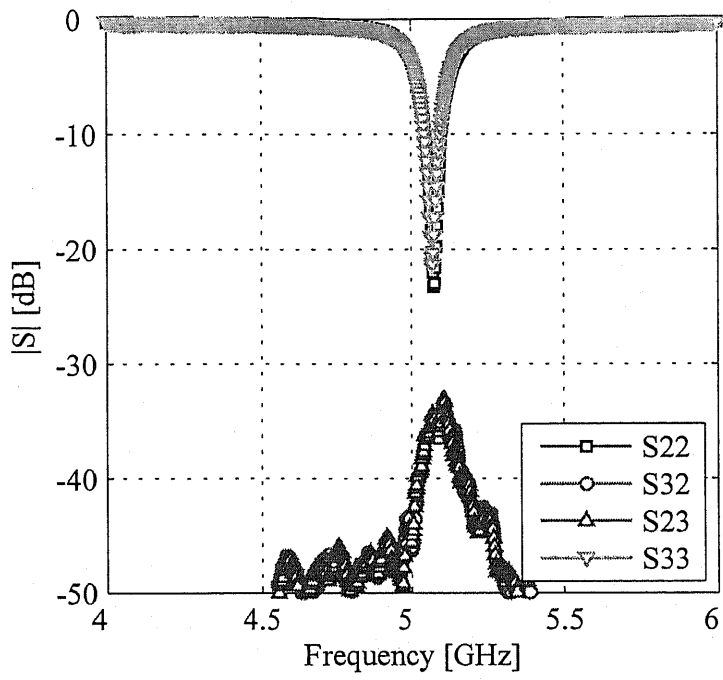
Figure 4.16: S parameters between #2 and #3.
