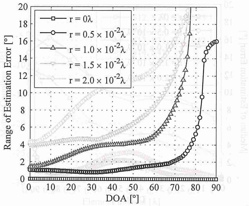
Figure 3.3: (c) Range of estimation error
