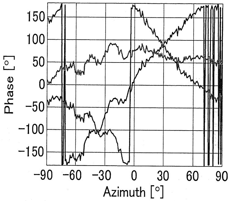
(c) Phase pattern of each element
