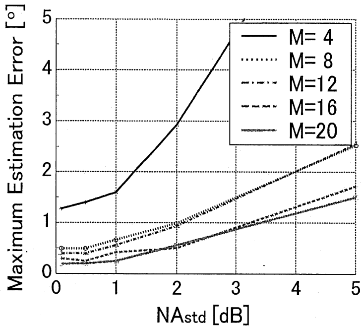
Figure 3.9: Maximum value of estimation error as a function of NA_{std} ( A_2: -30 dB) (simulation).
