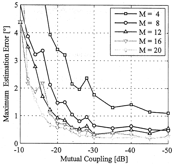
Figure 3.8: Maximum value of estimation error as a function of mutual coupling ( NA_{\text{std}} : 1 dB, N_{\phi_{\text{std}}} : 5^\circ ) (simulation).
