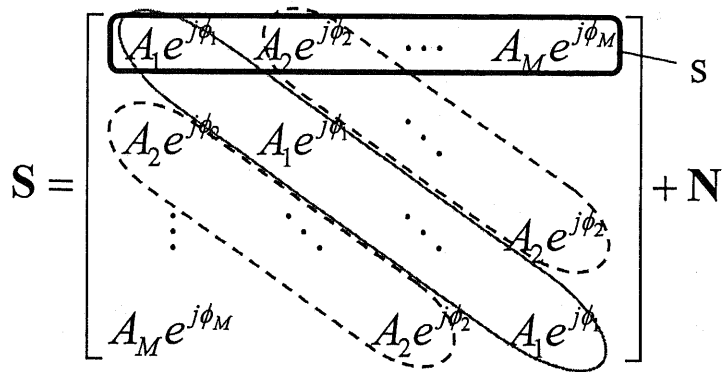
Figure 3.7: Scattering matrix.
