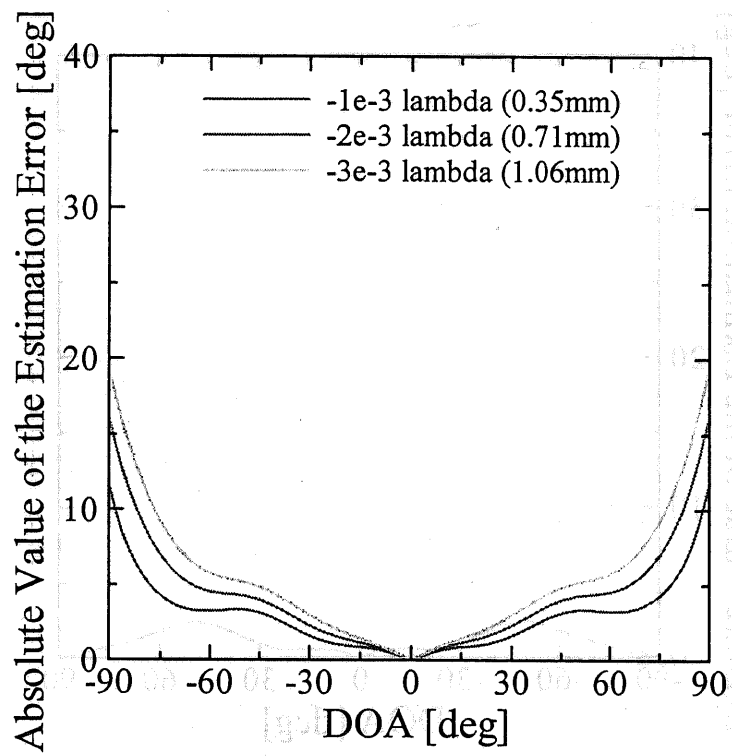
(c) Element interval of 0.5\lambda - \alpha
