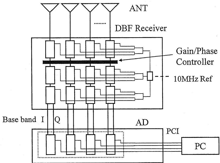
Figure 2.3: Composition of the DBF array antenna (initial).
