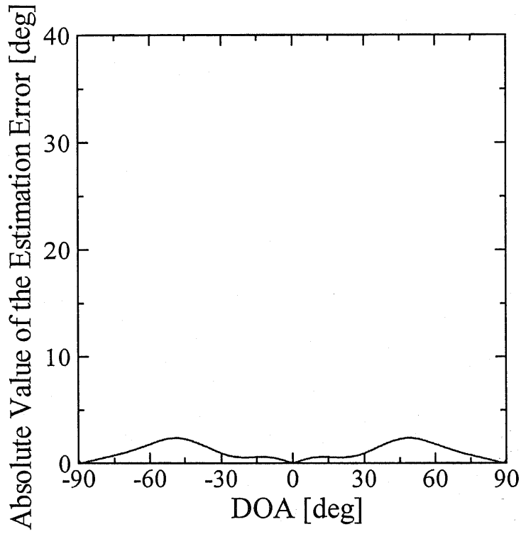
(a) Element interval of 0.5\lambda
