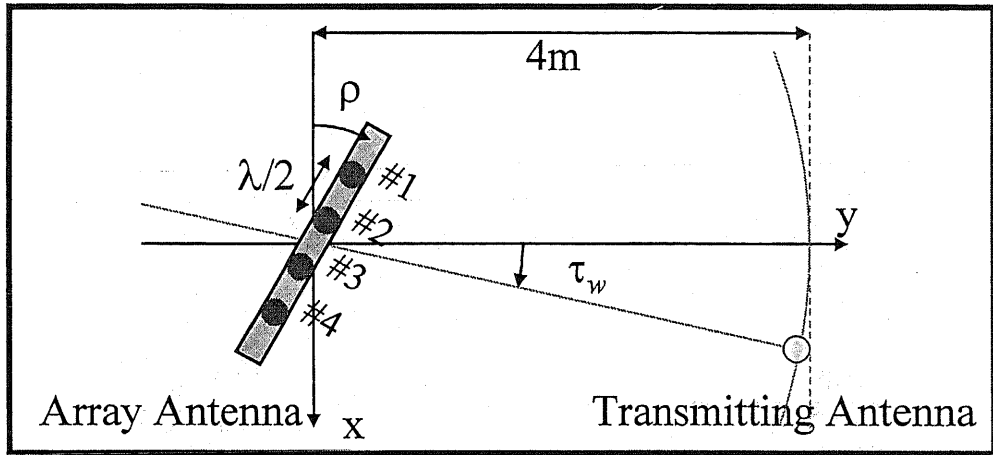
Figure 2.7: Evaluation of the array antenna system.
