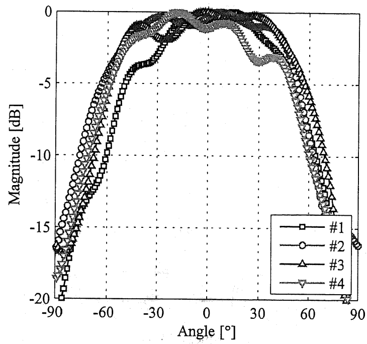
Figure 4.18: Element pattern (x-z plane) (measurement).
