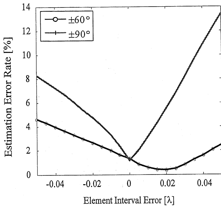
Figure 4.12: Estimation error rate (simulation).
