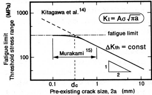
Fig. 4. Dependence of threshold conditions for fatigue crack growth of a microcrack on stress range.
