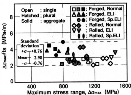
Fig. 5. Relationship between maximum stress range ( \Delta \sigma_{\max} ) and \Delta \sigma_{\max} \sqrt{f_s} for Ti-6Al-4V alloys.
