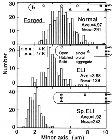
Fig. 3. \alpha grain size of the representative area shown in Photo. 1 a) c) e), and subsurface crack size of forged alloys.
